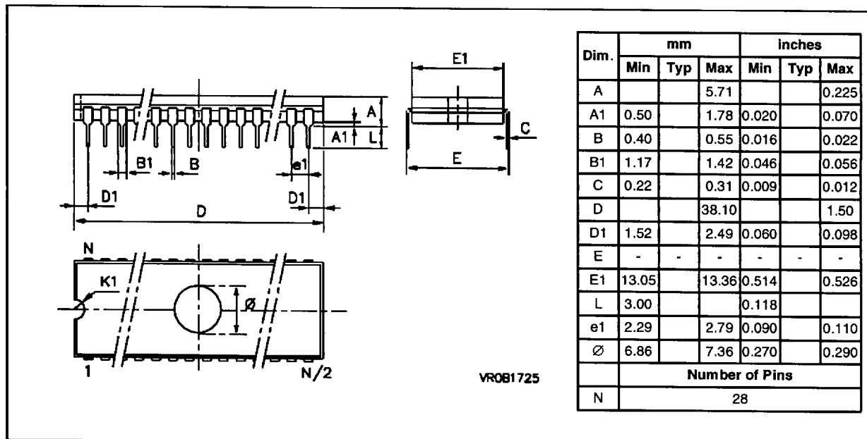
Figure 11. 28-Pin Ceramic Dual In Line Package, 600-mil Width
