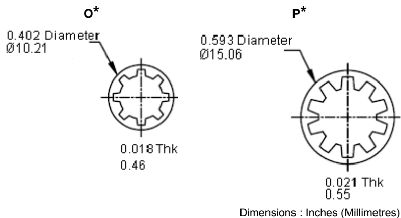
Lock Washer
