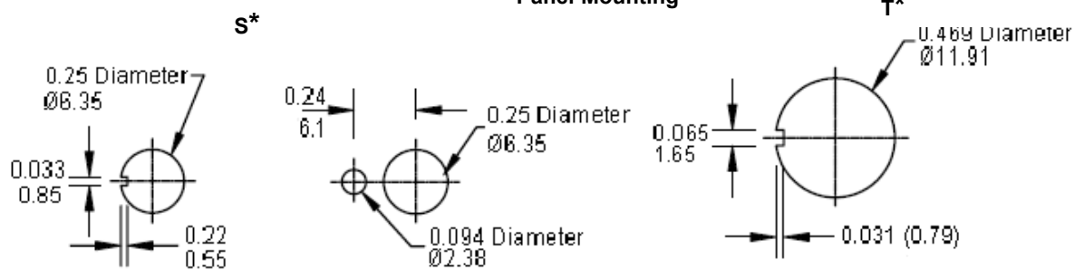
Panel Mounting
