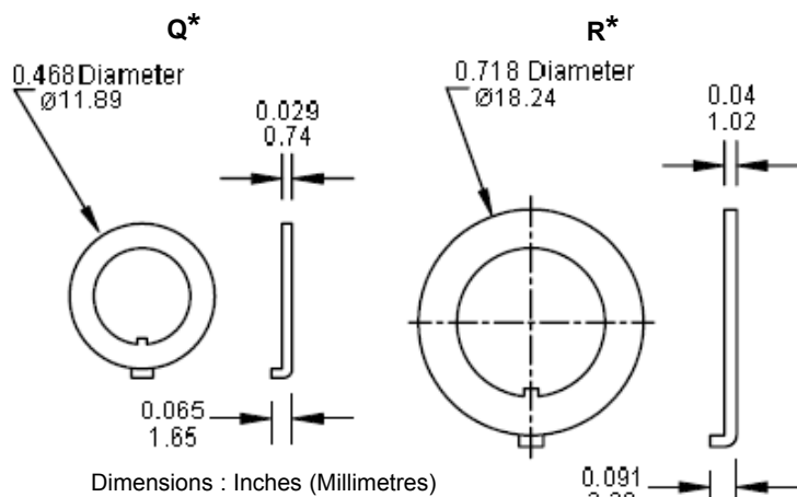
Panel Mounting
