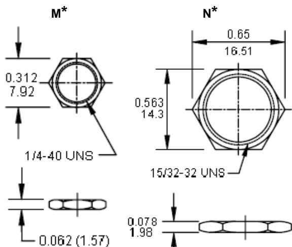
Standard Nuts
