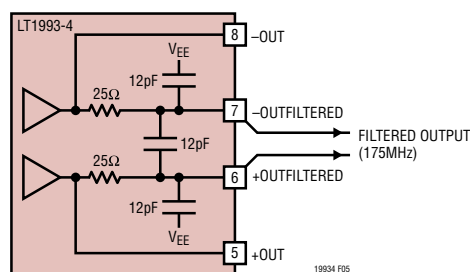
Figure 5. LT1993-4 Internal Filter Topology –3dB BW \approx 175MHz
