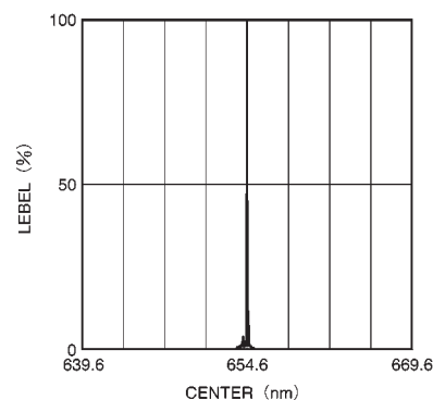
Fig.3 Emission spectrum
