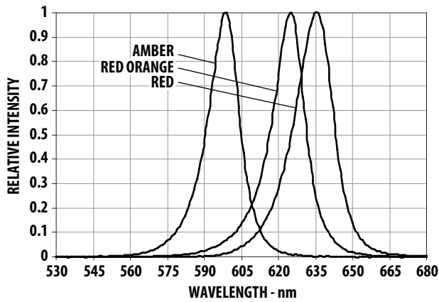
Figure 2. Relative Intensity vs. Wavelength for Red, Red Orange and Amber.
