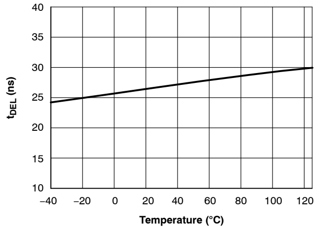
Figure 15. t DEL vs. Junction Temperature
