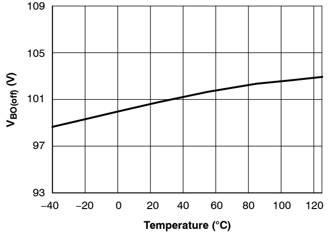
Figure 25. V BO(off) vs. Junction Temperature
