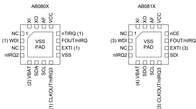
Figure 2. Pin Configuration Diagram
