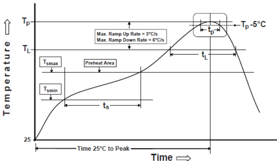
Figure 21. Reflow Soldering Diagram
