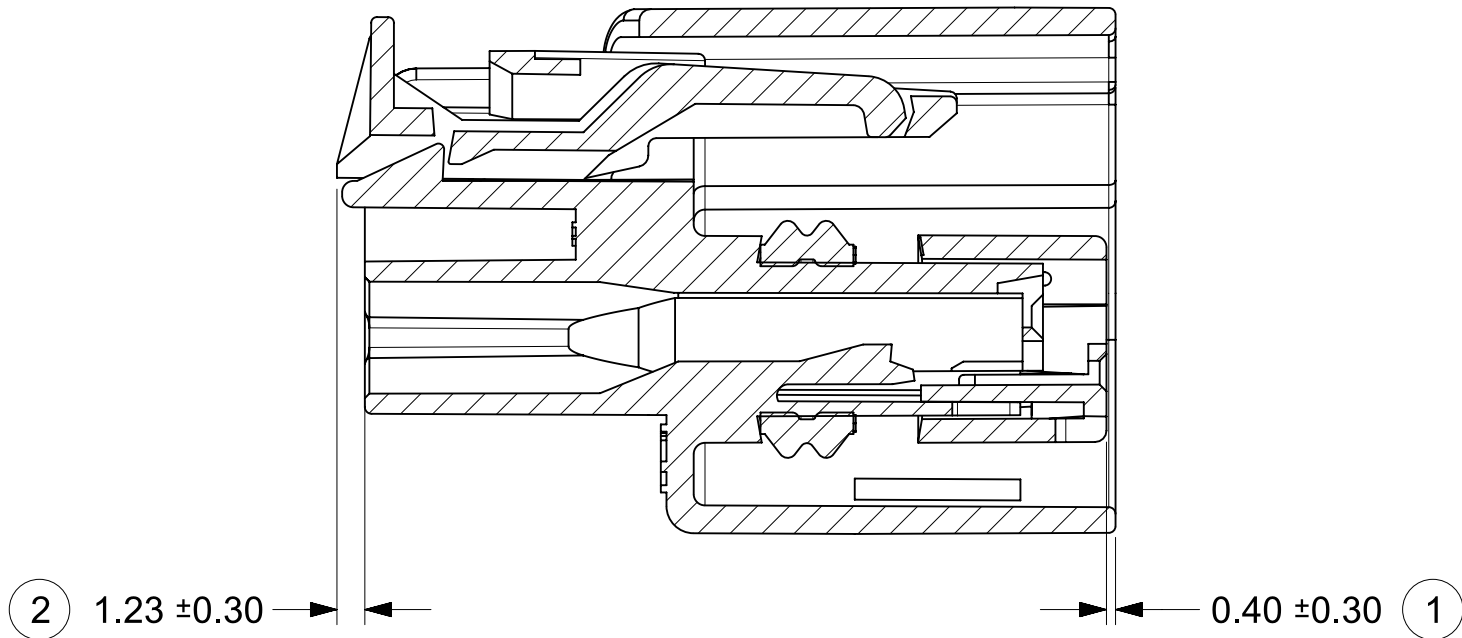
SECTION A-A TPA & CPA (OPTIONAL) SHOWN IN PRE-LOCK POSITION
