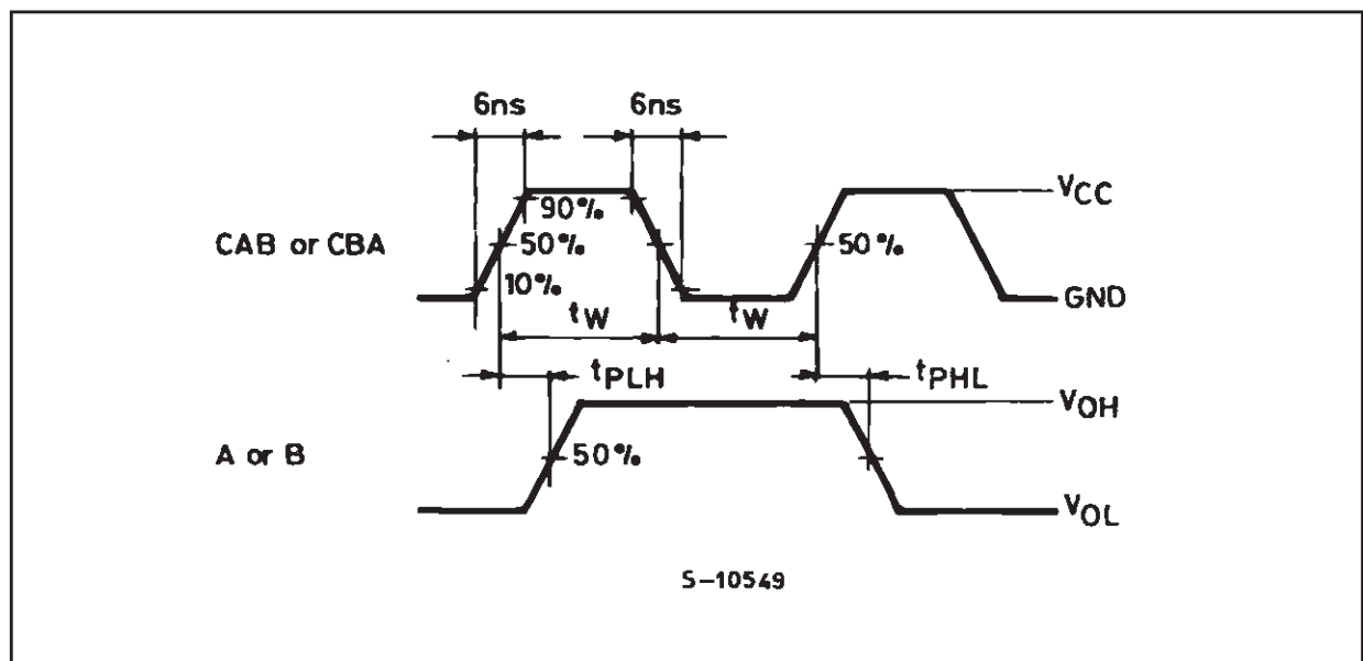
WAVEFORM 2 : PROPAGATION DELAY, MINIMUM PULSE WIDTH ( f=1\text{MHz} ; 50% duty cycle)
