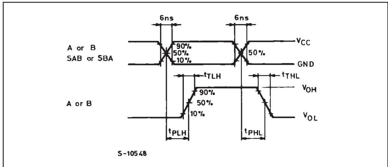
WAVEFORM 2 : PROPAGATION DELAY, MINIMUM PULSE WIDTH ( f=1\text{MHz} ; 50% duty cycle)
