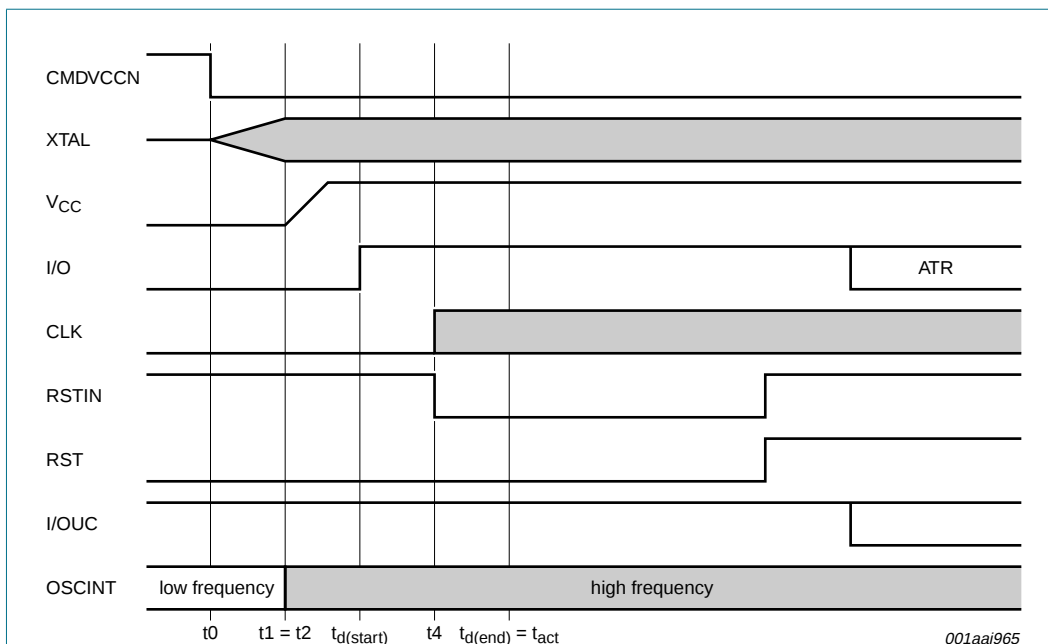
Fig 8. Activation sequence: CLK controlled by pin RSTIN with the crystal oscillator
