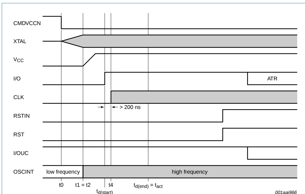
Fig 9. Activation sequence: CLK not controlled by pin RSTIN with the crystal oscillator
