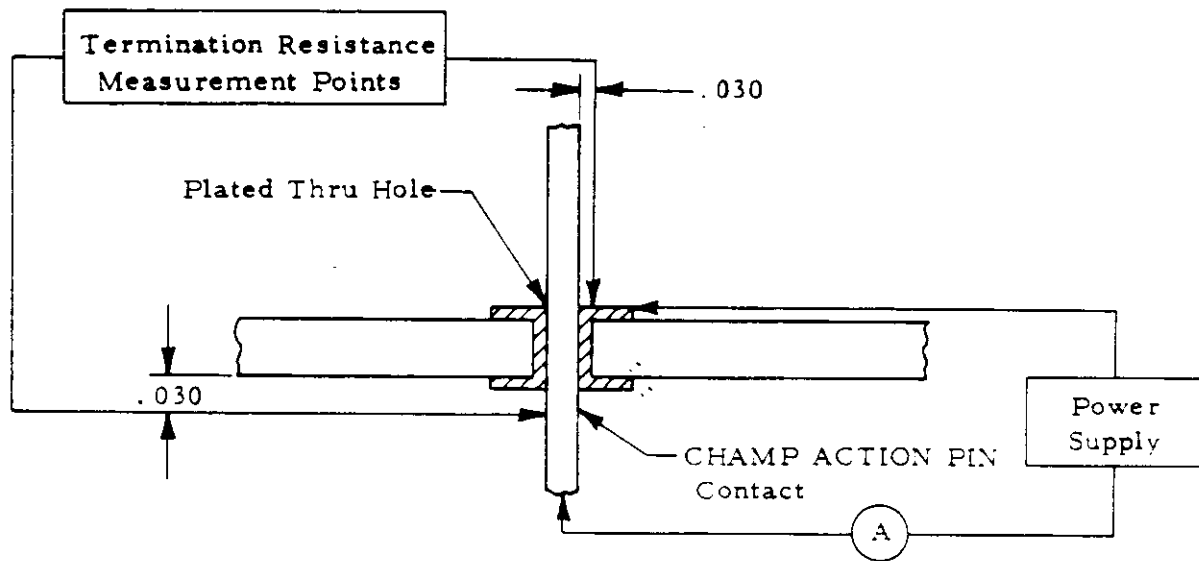
Figure 4 Resistance And Temperature Measurement Points
