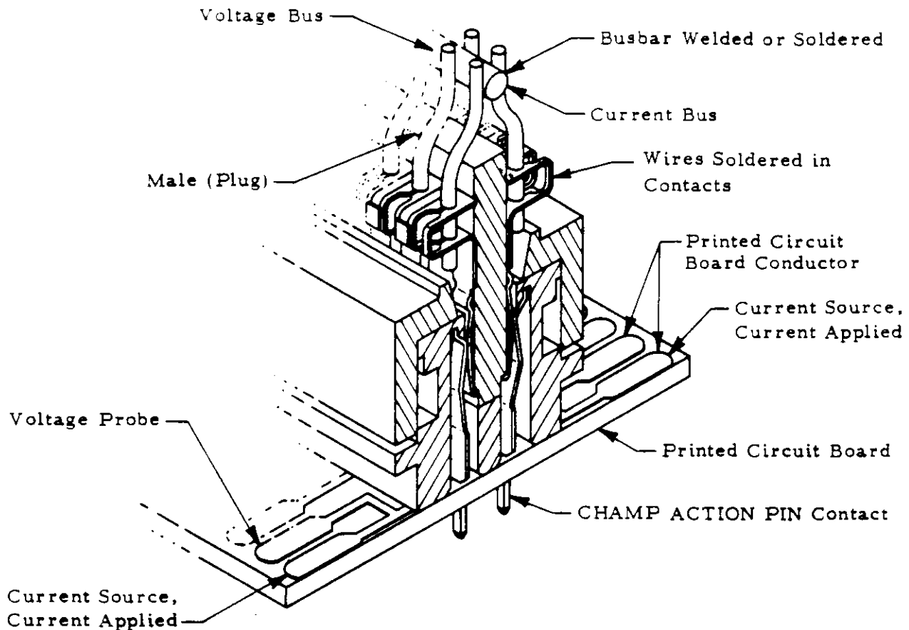
Figure 3 Mounting Mated Samples To Test Board For Millivolt Drop Measurements
