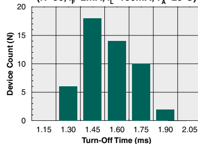
Typical Turn-Off Time (N=50, I_F=2\text{mA} , I_L=100\text{mA} , T_A=25^\circ\text{C} )
