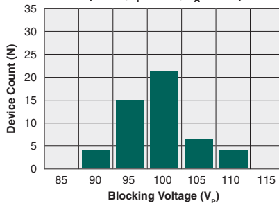
Typical Blocking Voltage Distribution (N=50, I_F=1\text{mA} , T_A=25^\circ\text{C} )
