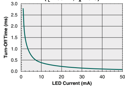
Typical Turn-Off Time vs. LED Forward Current ( I_L=100\text{mA} , T_A=25^\circ\text{C} )
