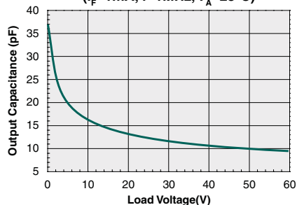
Output Capacitance vs. Load Voltage ( I_F=1\text{mA} , f=1\text{MHz} , T_A=25^\circ\text{C} )
