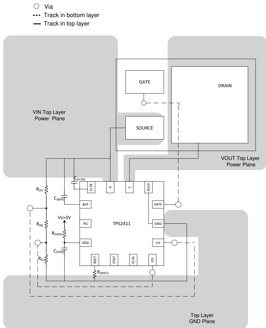
Figure 21. Example Layout
