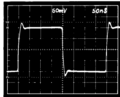
Figure 19c. Inverter Small Signal Pulse Response
