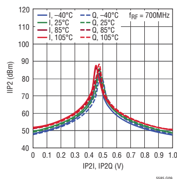
IIP2 vs IP2I, IP2Q Trim Voltage
