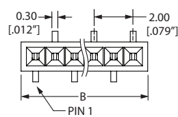
(SD) OPPOSITE BEND, APPLICABLE ON EVEN PIN COUNTS
