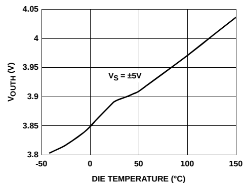
FIGURE 38. POSITIVE OUTPUT SWING vs TEMPERATURE
