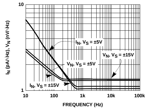
FIGURE 26. NOISE vs FREQUENCY
