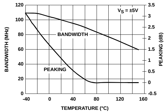
FIGURE 32. BANDWIDTH AND PEAKING vs TEMPERATURE
