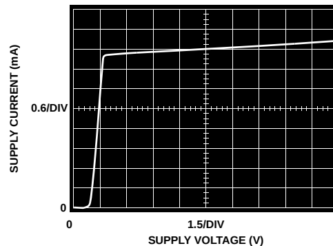
FIGURE 18. SUPPLY CURRENT vs SUPPLY VOLTAGE
