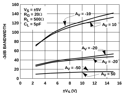
FIGURE 19. BANDWIDTH vs V_S
