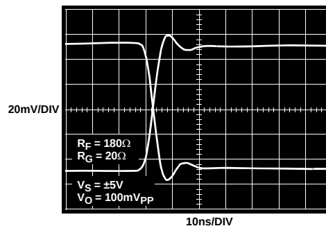
FIGURE 22. SMALL SIGNAL STEP RESPONSE
