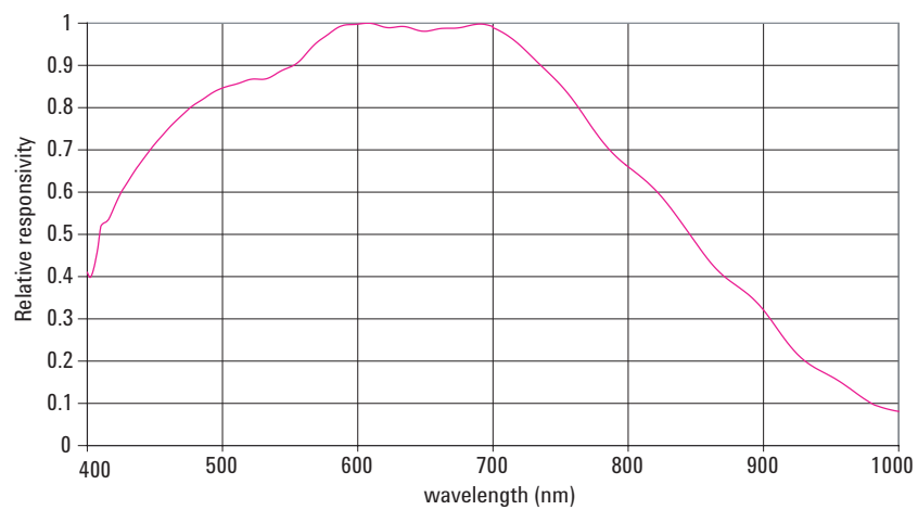
Figure 13. Relative responsivity
