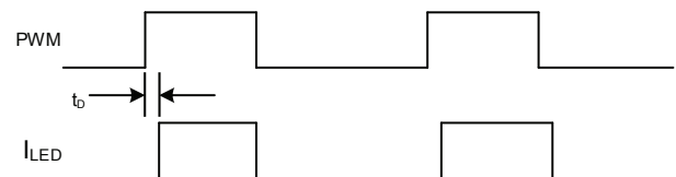
Figure 13. Propagation delay from the PWM signal rising edge to I_{\text{LEDx}} reaching the 90% level
