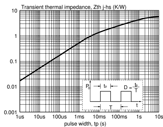
Fig.11. Transient thermal impedance; Z_{th\ j-hs} = f(t_p) .
