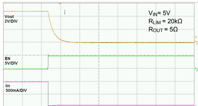
Figure 4 Turn-Off Delay and Fall Time
