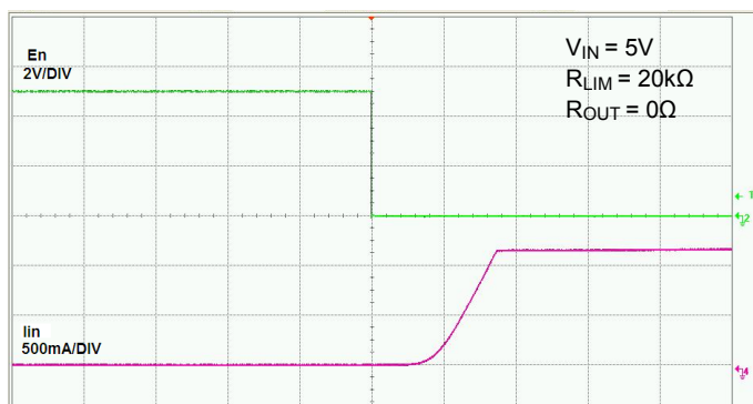
Figure 5 Device Enabled into Short-circuit
