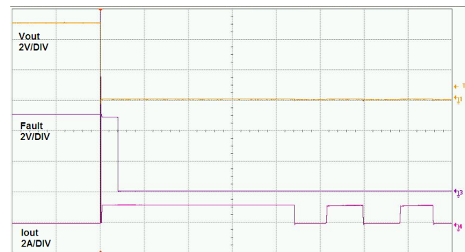
Figure 8 Extended Short-Circuit into Thermal Cycles
