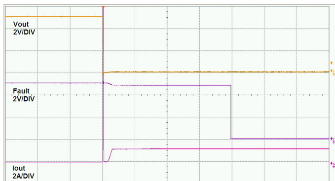
Figure 7 Short-Circuit Current Limit Response
