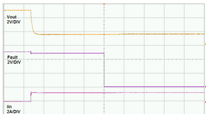
Figure 6 No Load to 1Ω Transient Response
