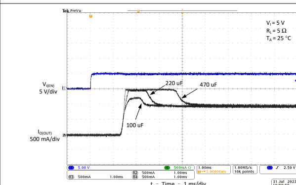
Figure 6-16. Inrush Current With Different Load Capacitance
