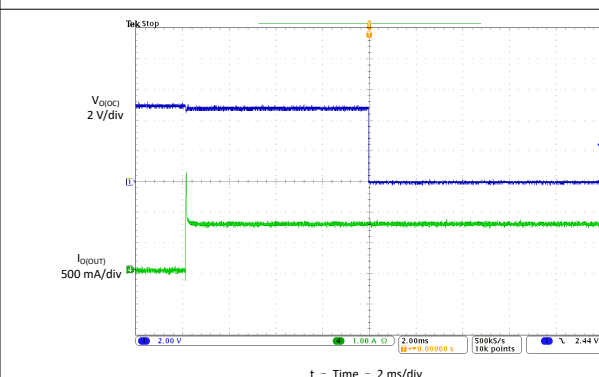
Figure 6-18. 2-Ω Load Connected to Enabled Device
