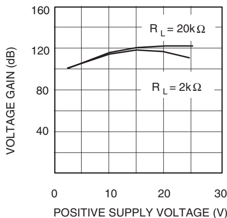
Figure 15. Voltage gain
