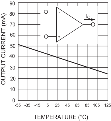
Figure 4. Current limiting
