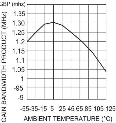
Figure 6. Gain bandwidth product
