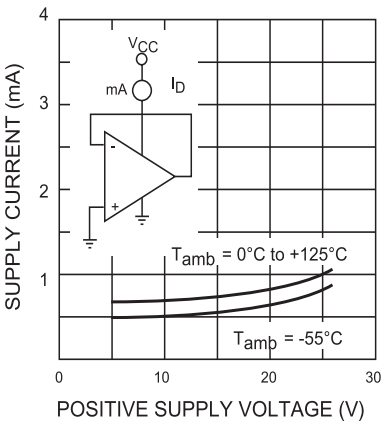
Figure 5. Supply current
