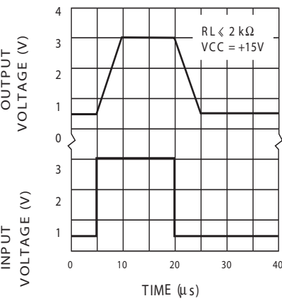
Figure 7. Voltage follower pulse response
