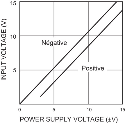
Figure 3. Input voltage range
