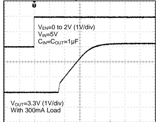
Start-Up Time
