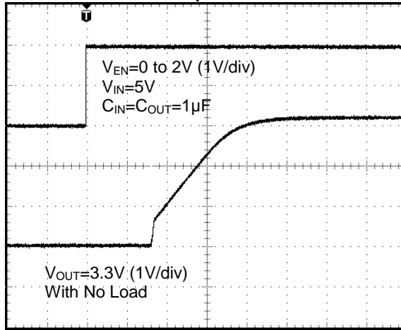
Start-Up Time
