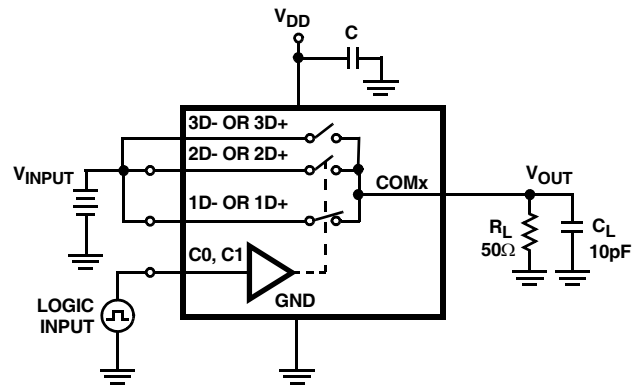
FIGURE 1. SWITCHING TIMES
