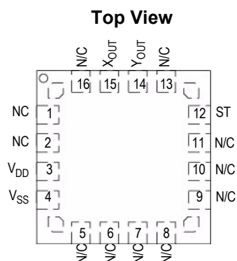
Figure 4. Pinout Description
