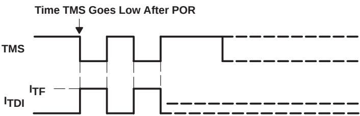
Figure 20. Fuse Check Mode Current, MSP430C33x
