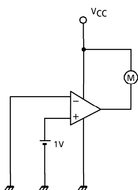
(3) I_{LEAK}
