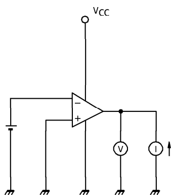
(5) I_{SINK}, V_{OL}
