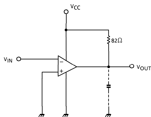
(6) t_{rsp}
