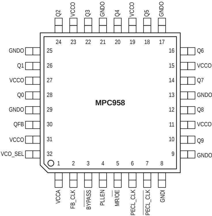
Figure 2. 32-Lead Pinout (Top View)
