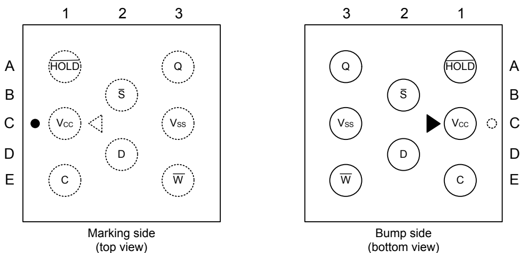
Figure 3. WLCSP connections
