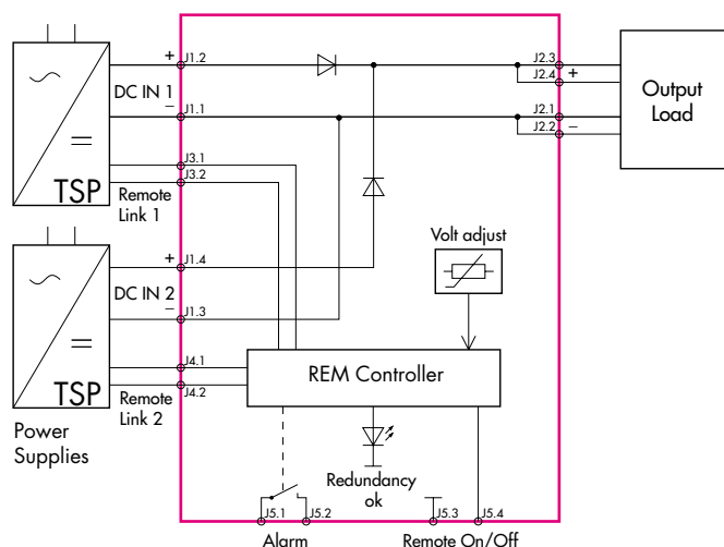
Function Diagram
