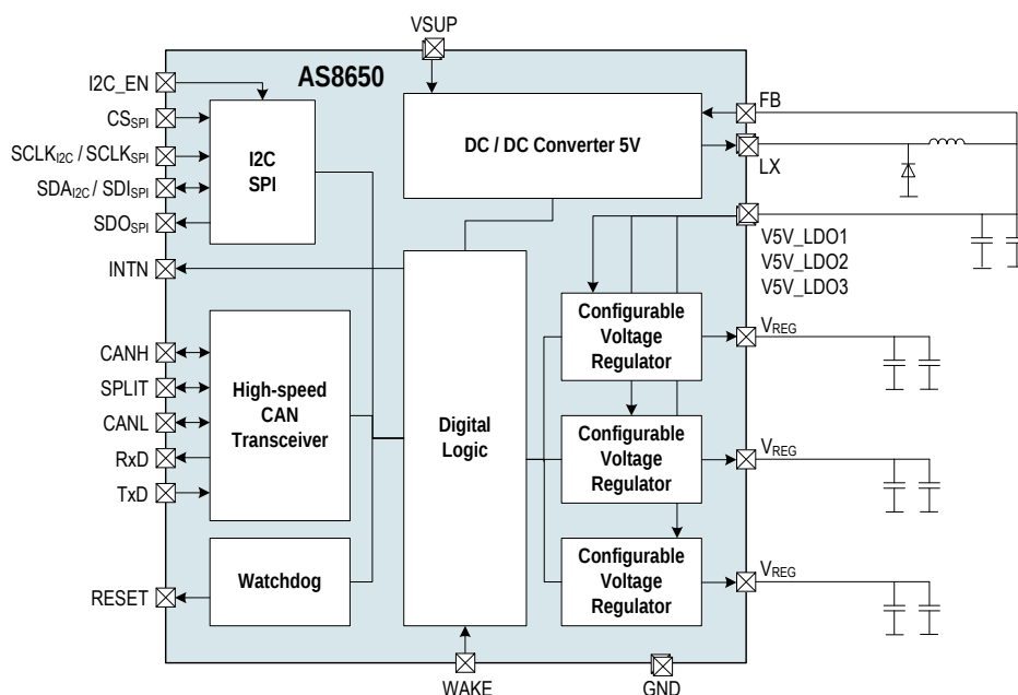
Figure 1. AS8650 Block Diagram
