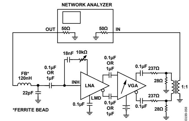
Figure 58. Test Circuit—Group Delay vs. Frequency for Two Values of AC Coupling
