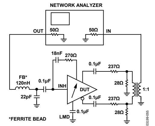
Figure 55. Test Circuit—Gain and Bandwidth Measurements
