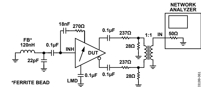
Figure 61. Test Circuit—Short-Circuit, Input-Referred Noise
