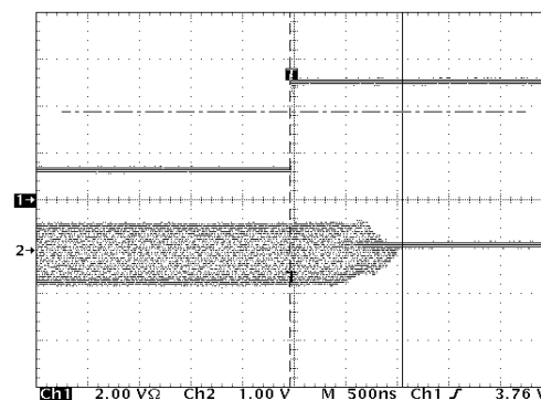
FIGURE 16. DISABLED RESPONSE
