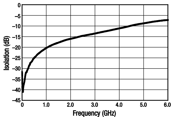
Figure 4. Isolation vs Frequency ( V_R = 0 V)
