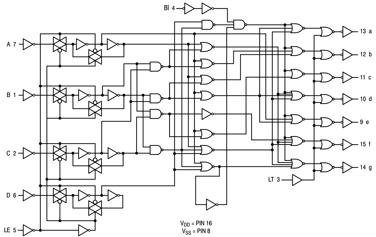
Figure 3. Logic Diagram
