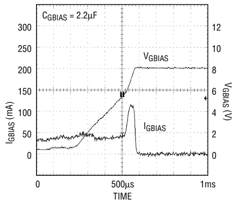
G_{BIAS} vs I_{GBIAS} (Charging 2.2μF)
