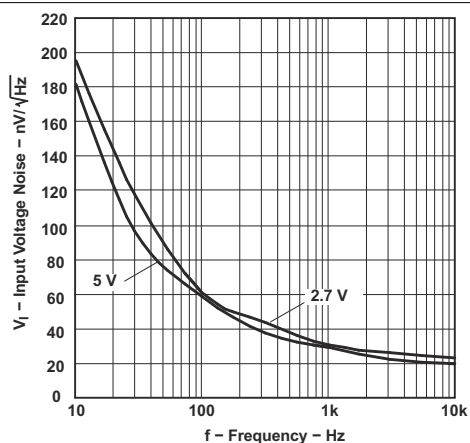
Figure 5-18. Input Voltage Noise vs Frequency
