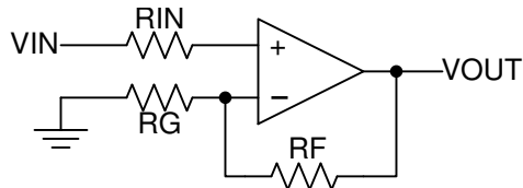
Figure 9-2. Operational Amplifier Schematic for Noninverting Configuration
