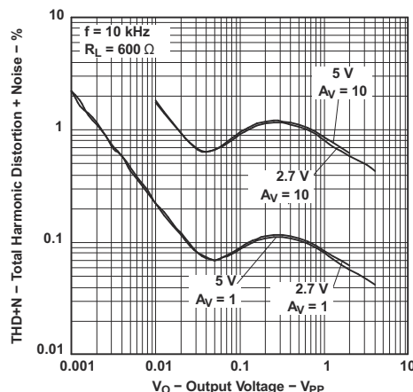
Figure 5-20. Total Harmonic Distortion + Noise vs Output Voltage
