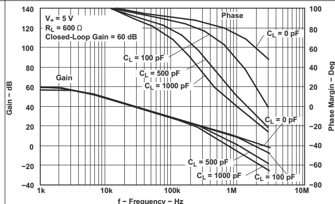
Figure 5-22. Gain and Phase Margin vs Frequency
