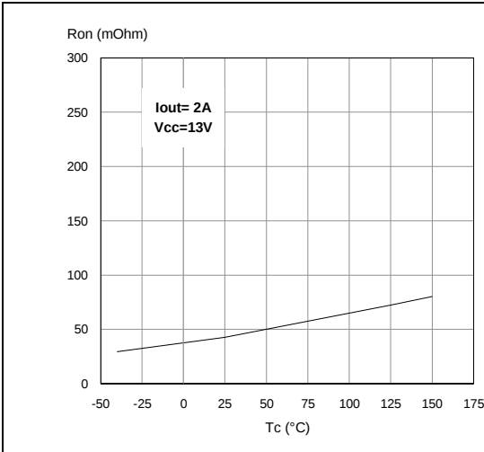
Figure 20. On-state resistance vs. T_{case}
