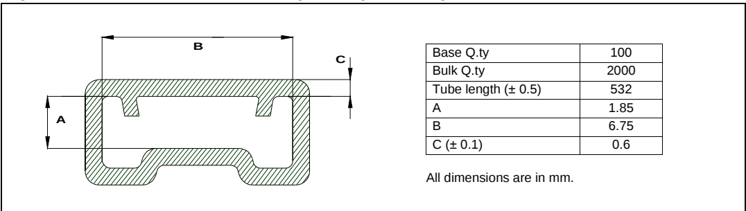
Figure 37. PowerSSO-12 tube shipment (no suffix)
