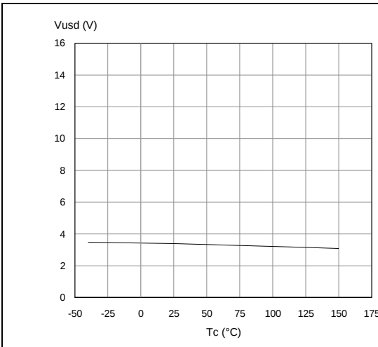
Figure 22. Undervoltage shutdown
