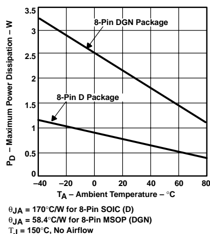
Figure 113. Maximum Power Dissipation vs Ambient Temperature
