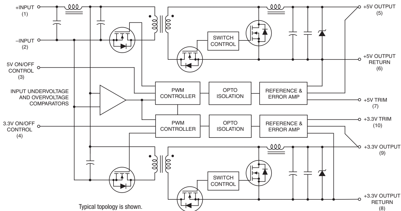
Figure 1. Simplified Schematic
