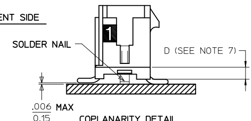
COPLANARITY DETAIL SEE NOTE #6
