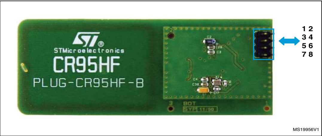
Figure 3. PLUG-CR95HF-B connector
