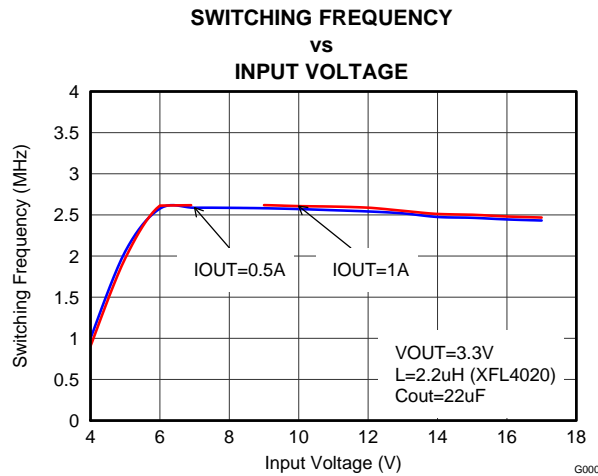
Figure 19. Switching Frequency
