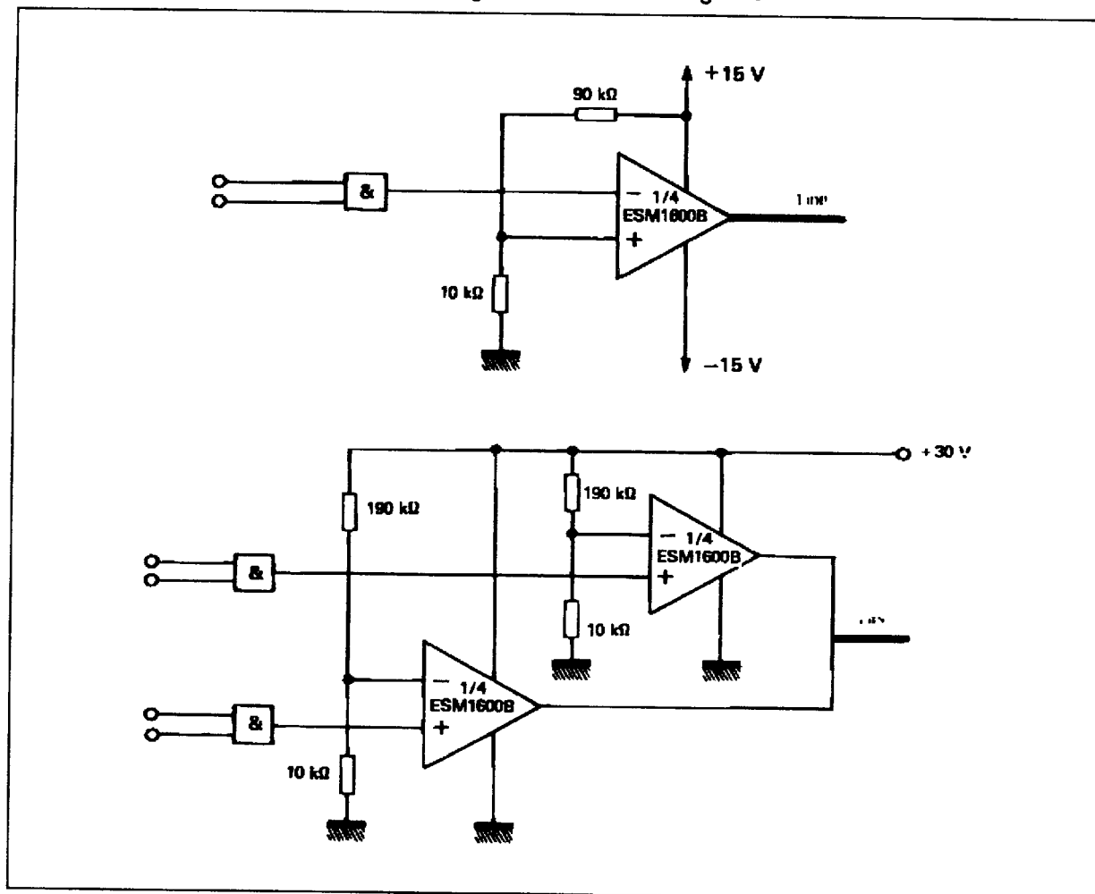
Figure 6 : Reception of Highly Noisy Signals.
