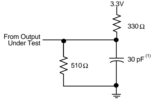
PROPAGATION DELAY LOAD CIRCUIT
