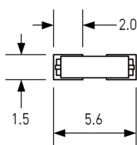
Pad sizes
