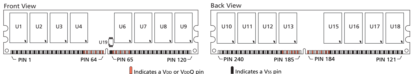
Figure 2: Pin Locations
