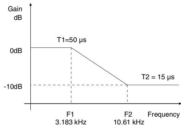
Figure 13. De-Emphasis Curve
