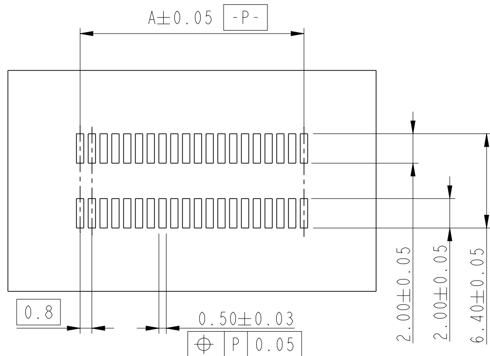
RECOMMENDED PCB LAYOUT WITHOUT PEGS AND HOLDDOWN
